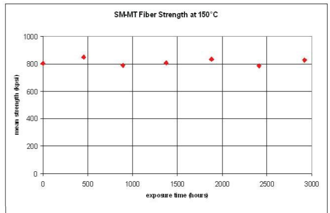
Strength of Fiber Aged at 150°C (2,900 hours)
