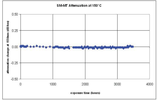
Aged Attenuation at 150°C (3,500 hours)
