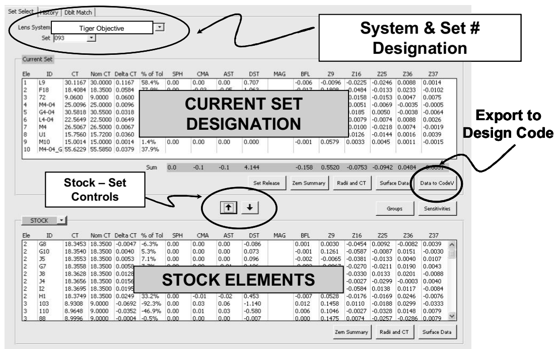
Fig. 3. Project Element Selection Interface in LMD
