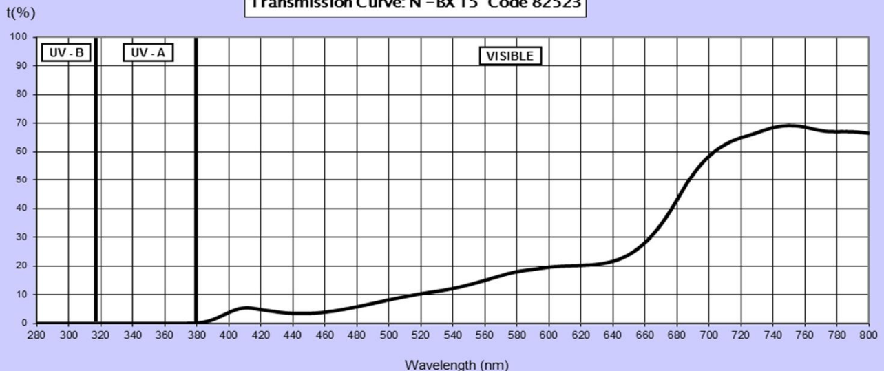
Transmission Curve: N -BX 15 Code 82523
