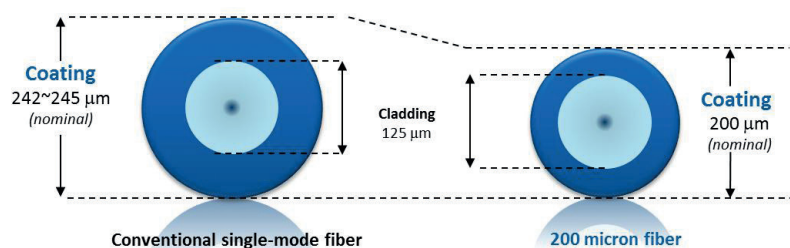
Figure 1 Cross sections of conventional and 200-micron fibres
