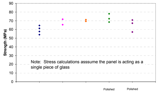
AUO 13.3 inch Panel 4 Point Bend Results (Edge Strength)
