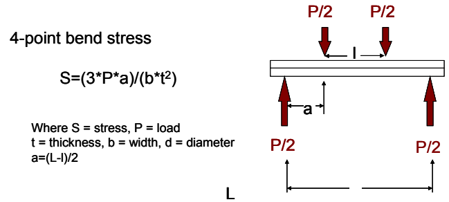
Figure 6. Schematic of four point bend test.
