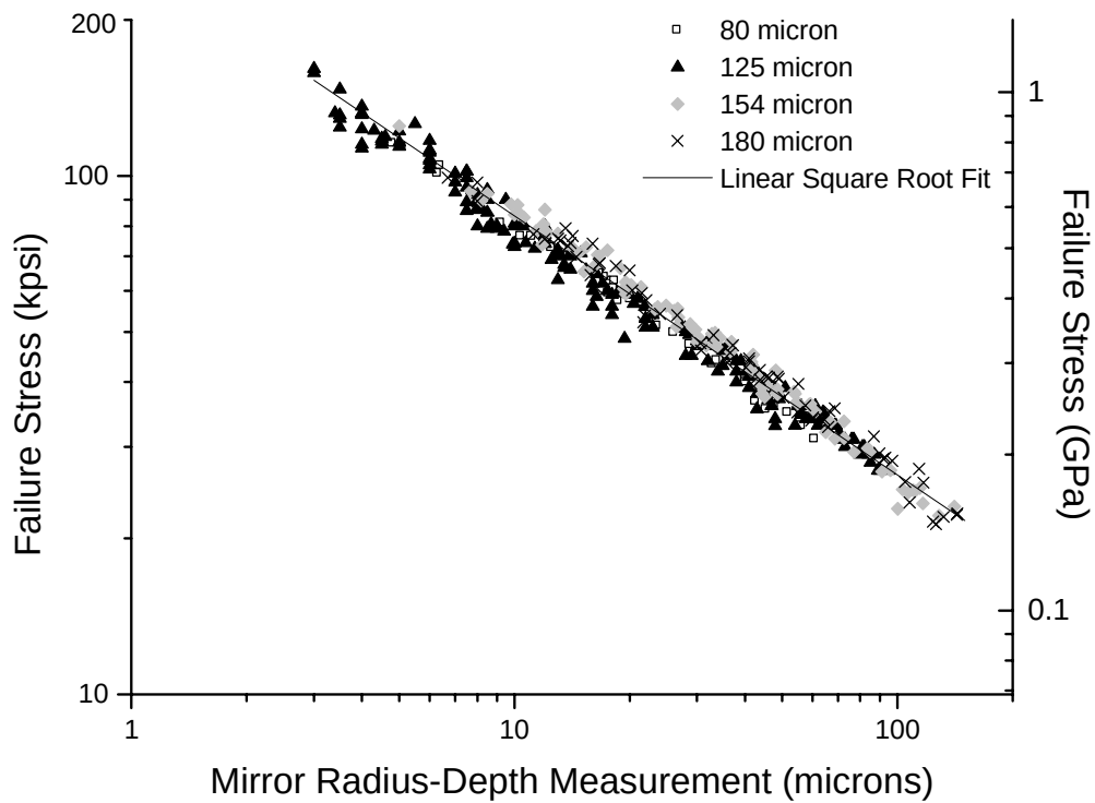
Figure 7. Plot showing mirror radius-depth ( r_d ) measurement values versus failure stress for various diameter fibers.
