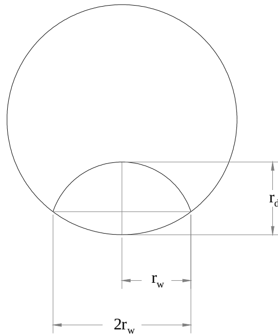
Figure 2. Schematic showing mirror radius-depth ( r_d ) and radius-width ( r_w ) measurements on a fiber break end.
