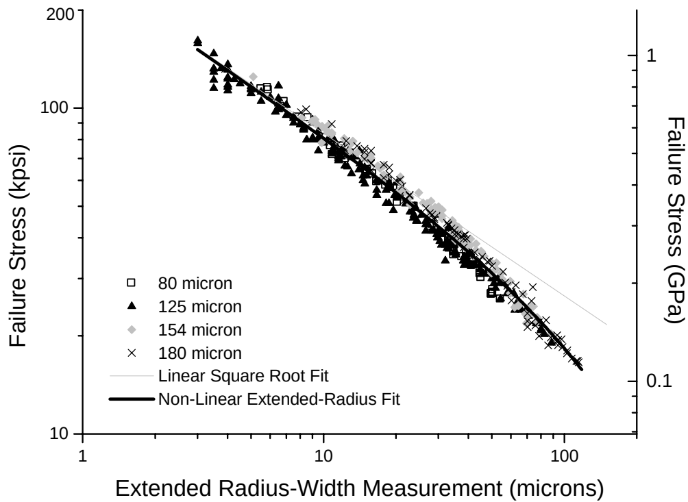
Figure 9. Plot showing extended radius-width ( r_x ) measurement values versus failure stress for various diameter fibers.
