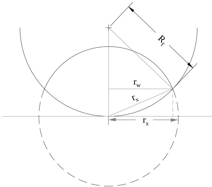
Figure 5. Schematic showing the extended radius-width measurement ( r_x ) and a fiber of radius ( R_f ).
