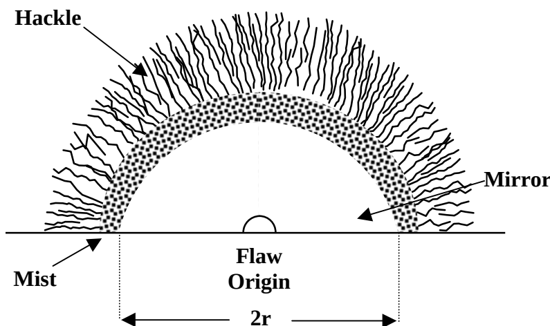
Figure 1. Schematic showing typical glass surface features that form during failure.
