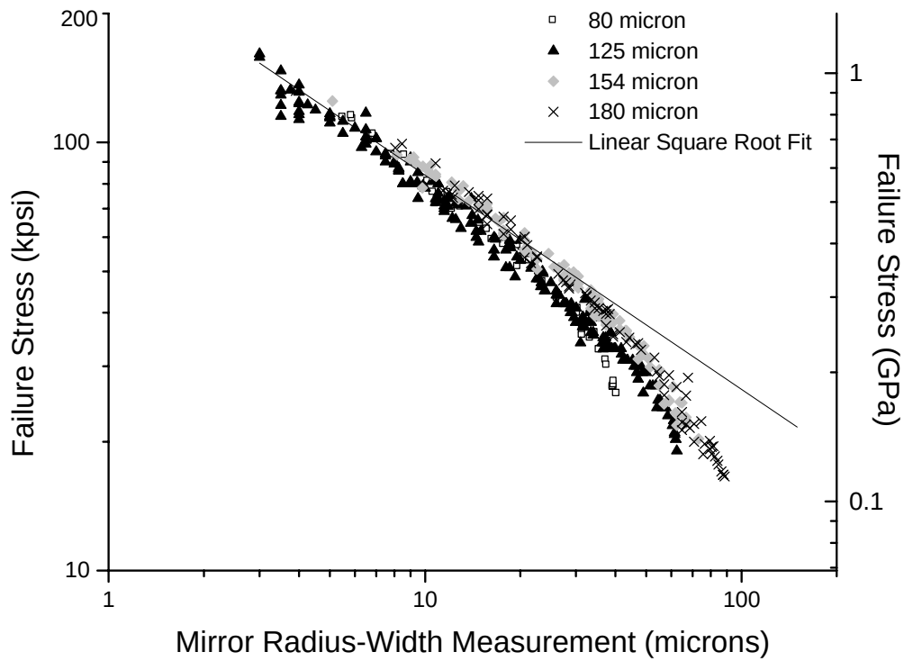
Figure 8. Plot showing mirror radius-width ( r_w ) measurement values versus failure stress for various diameter fibers.
