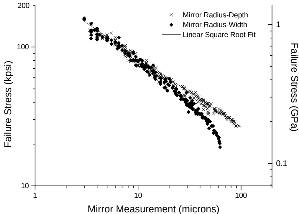
Figure 3. Plot showing the mirror radius-depth ( r_d ) and radius-width ( r_w ) measurement values versus failure stress for 125 \mu\text{m} diameter fiber.
