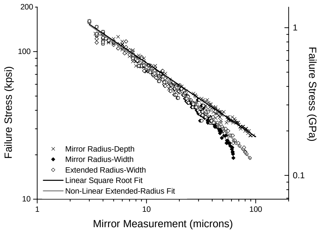
Figure 6. Plot showing mirror measurement values versus failure stress including the extended radius-width ( r_x ) data.
