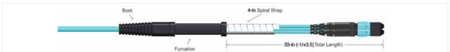
EDGE Solutions Trunk Cable Configuration | Drawing ZA-3496
