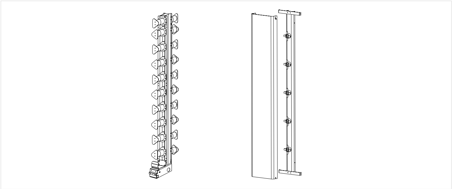
ECL-IBD-7-1 Inter-Bay Storage Units and ECL-EC-7 End Cap | Drawings ZA-1883 and ZA-1917
