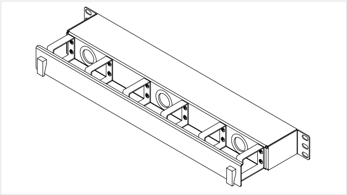
ECL-J1U Jumper Management Panel | Drawing ZA-1547
