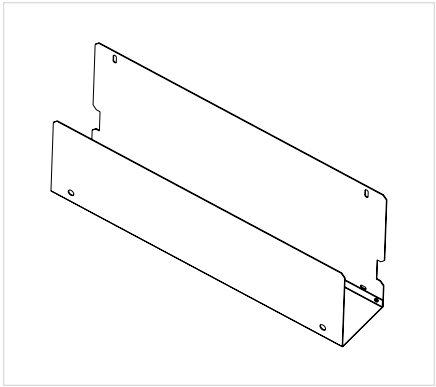
UDF-JBX Deep Bottom Trough Drawing ZA-2148
