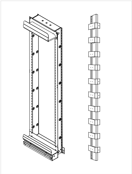
ECL-BAY-7 Network Bay and UDF-RBS-07-075 Rear-Bay Storage Unit | Drawings ZA-1546 and ZA-1265
