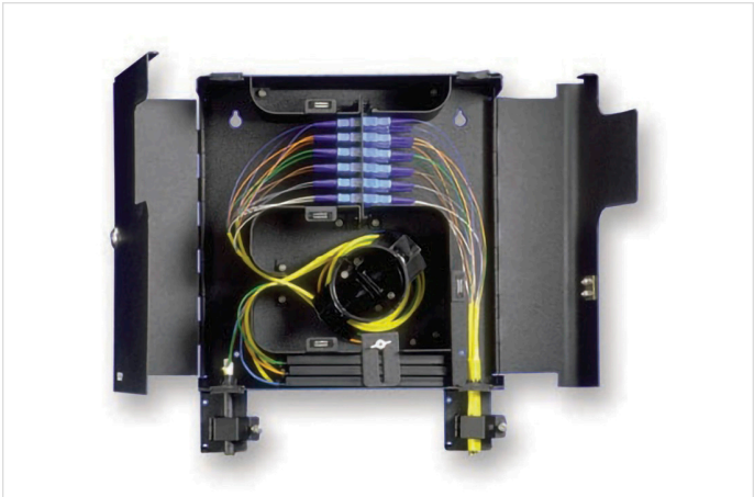
Open ECL-W3P-L Wall-Mountable Housing Showing Customer and Provider Access | Photo ICH149
