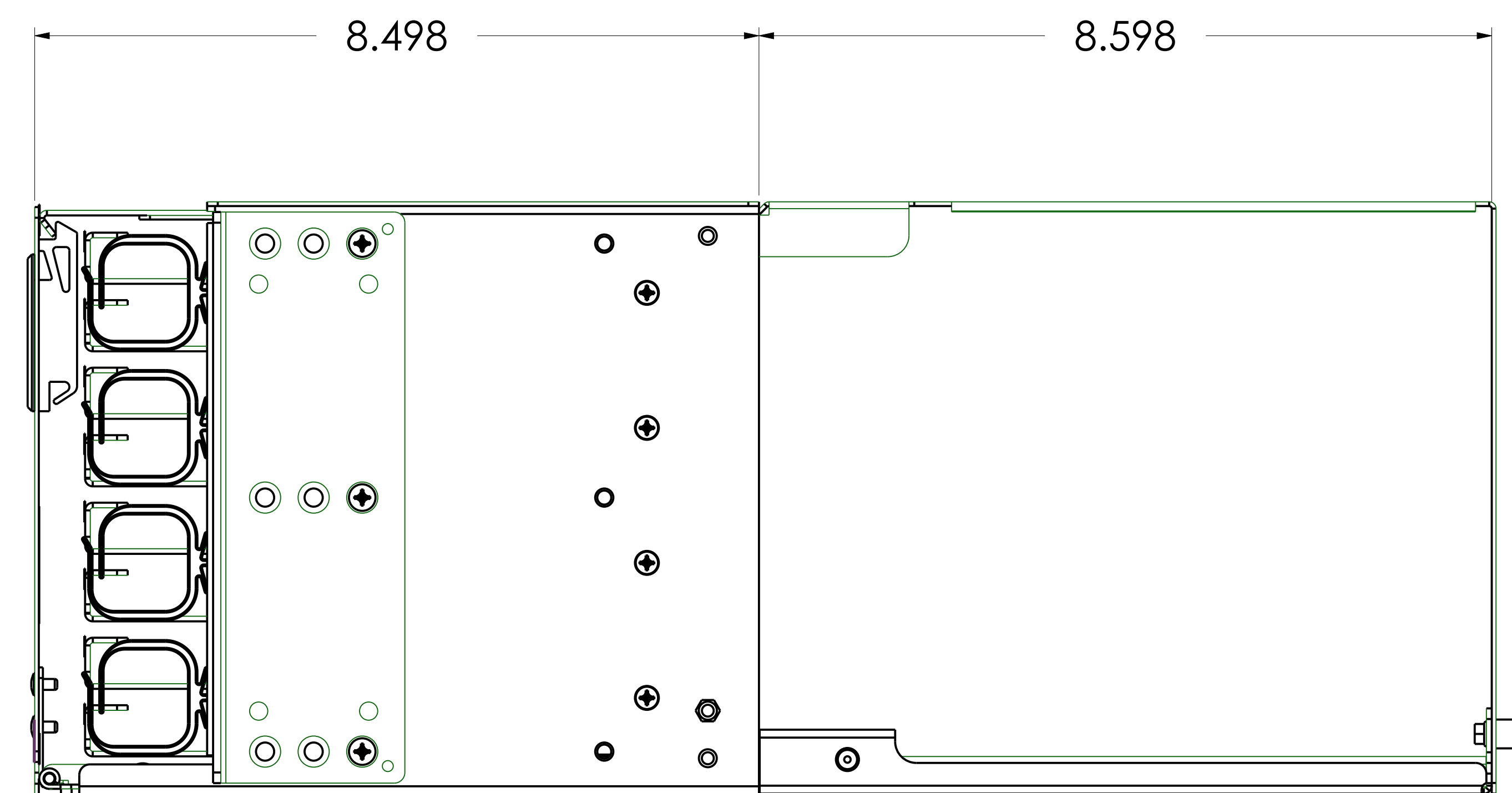
RIGHT SIDE
