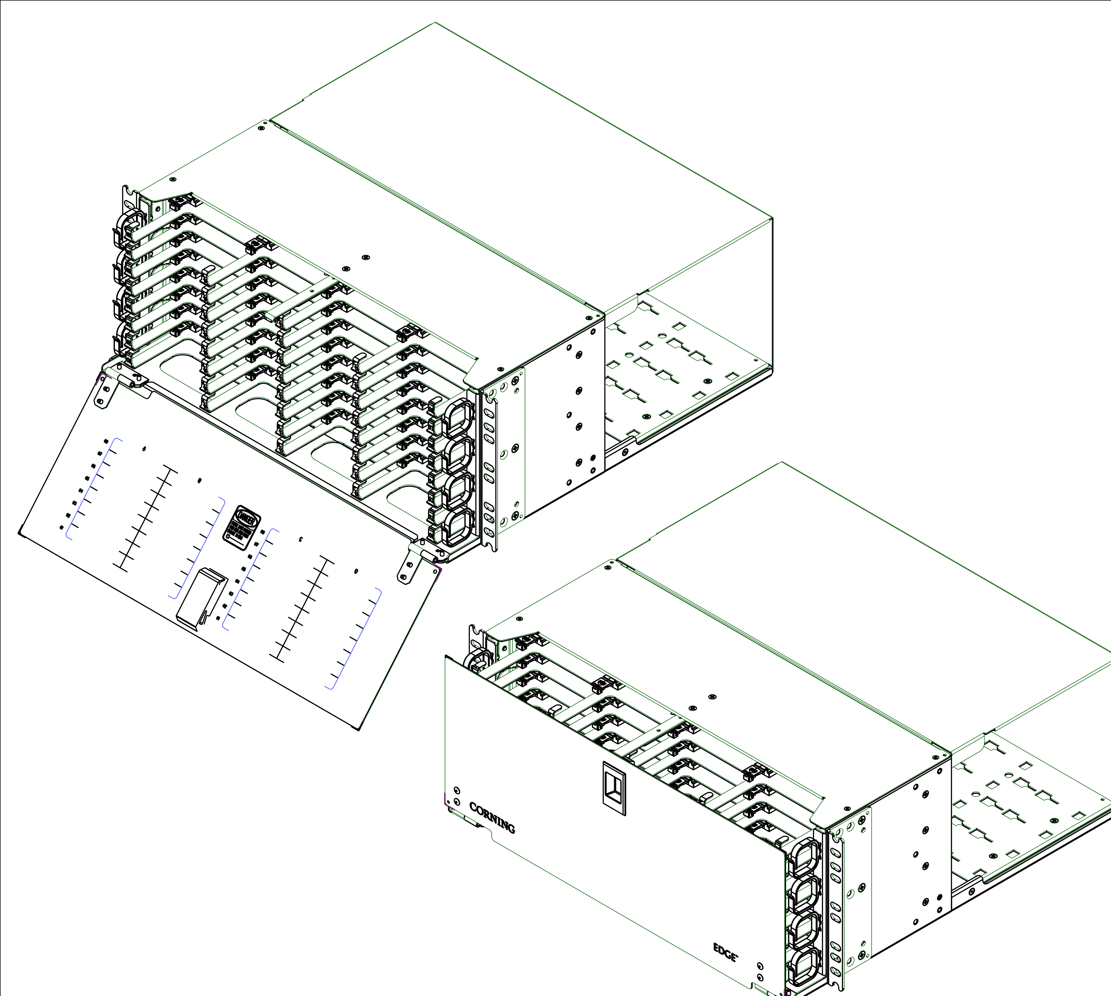
FRONT SIDE
