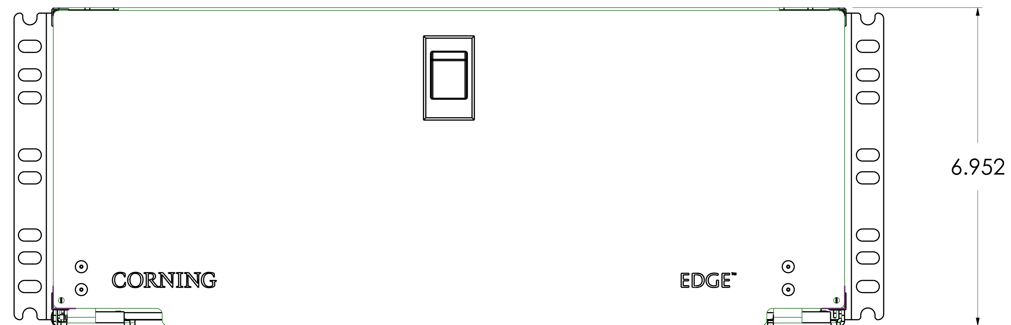
FRONT SIDE
