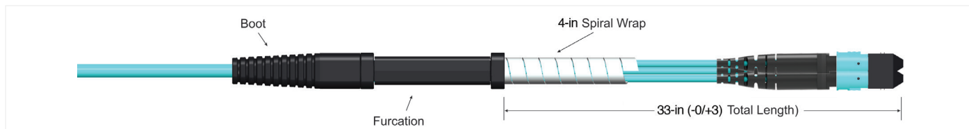
EDGE Solutions Trunk Cable | Drawing ZA-3496
