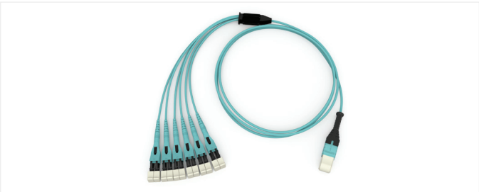
EDGE MTP to LC Uniboot Harness, non-staggered | Photo REN7795
