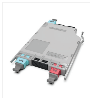
MTP to MTP Multimode TAP Module | Photo REN3559
