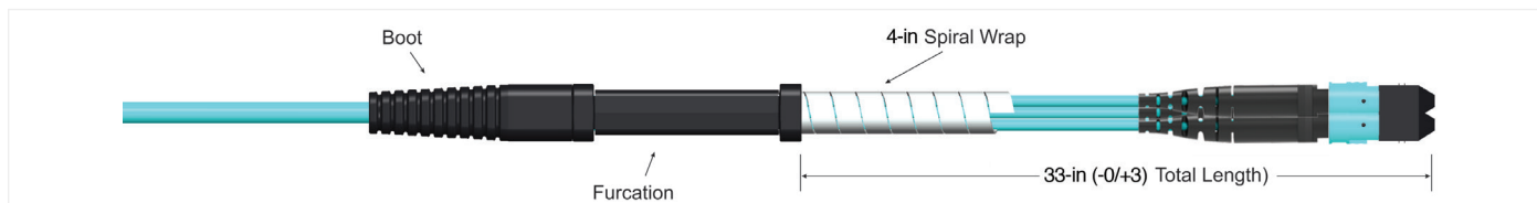
EDGE Solutions Trunk Cable | Drawing ZA-3496
