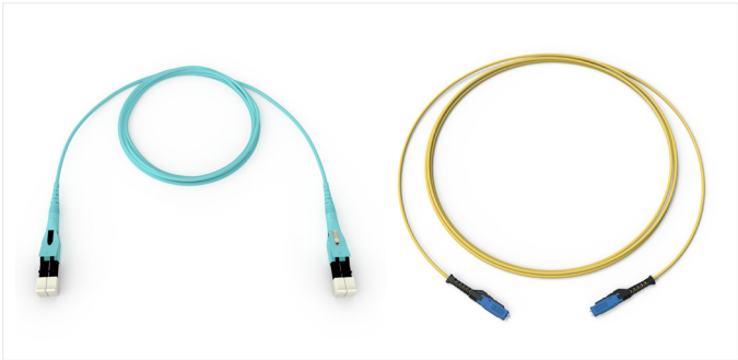
Reverse Polarity LC Uniboot and MDC Duplex Patch Cords | Photos REN6462 and REN8003
