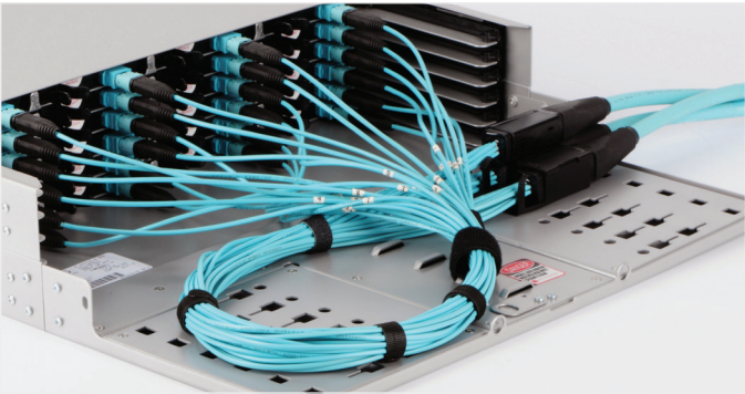
EDGE-02U Rack-Mount Rear Side | Photo LAN7314
