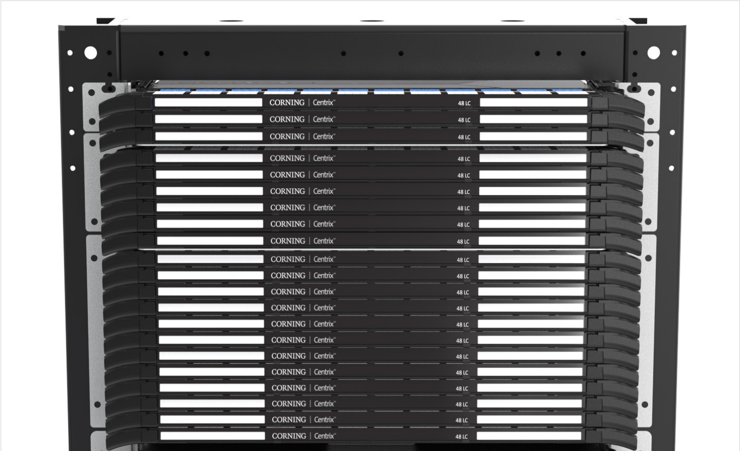
CTX-XL 1U with (3) 48 port LC cassettes, CTX-XL 2U with (6) 48 port LC cassettes, CTX-XL 4U with (12) 48 port LC cassettes
