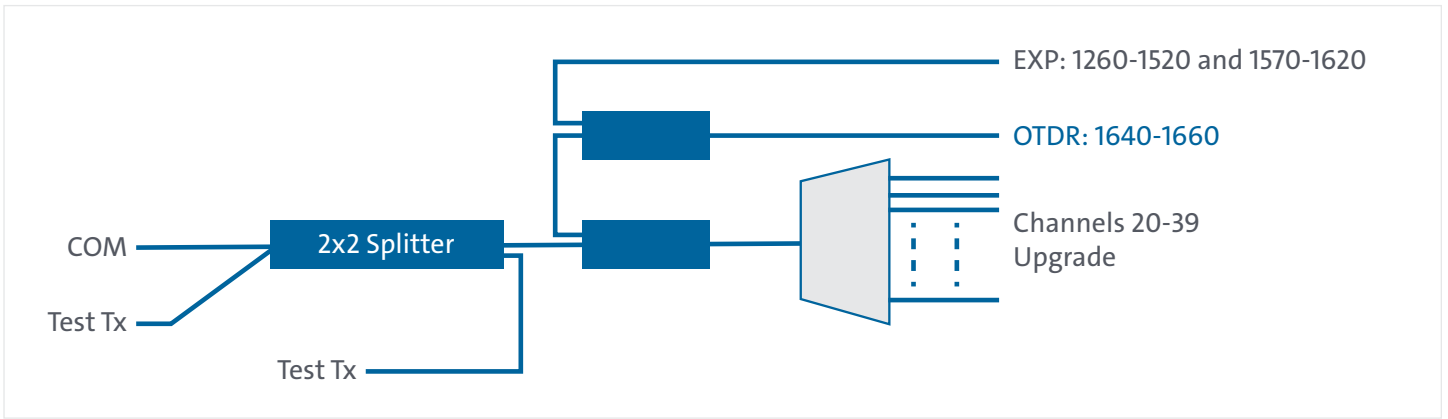
Optical Layout
