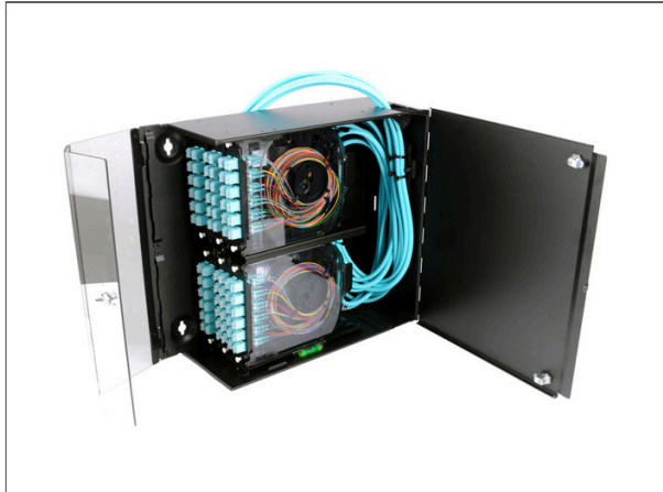
Wall-Mountable Closet Housing (WCH), holds 6 CCH connector panels/cassettes
