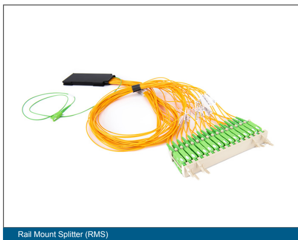
Rail Mount Splitter (RMS)
