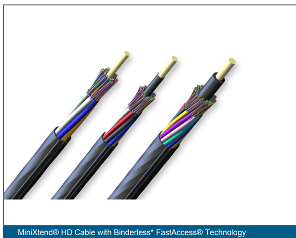
MiniXtend® HD Cable with Binderless* FastAccess® Technology
