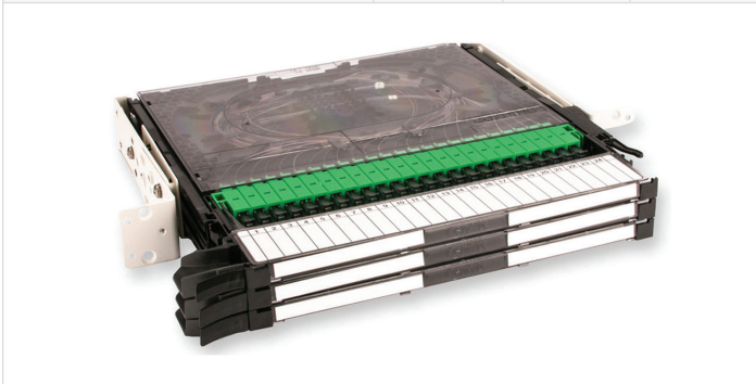
Centrix CTX-S1U Housing with 3 Cassettes
