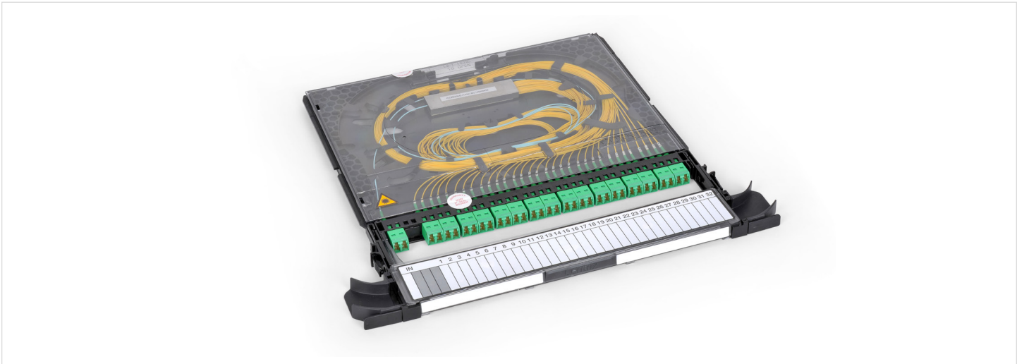
Centrix™ Splitter Cassette | Photo CRR3810
