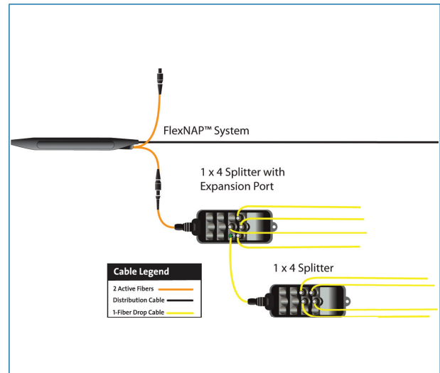
OptiSheath MultiPort Splitter Terminals with the FlexNAP System | Drawing ZA-3672
