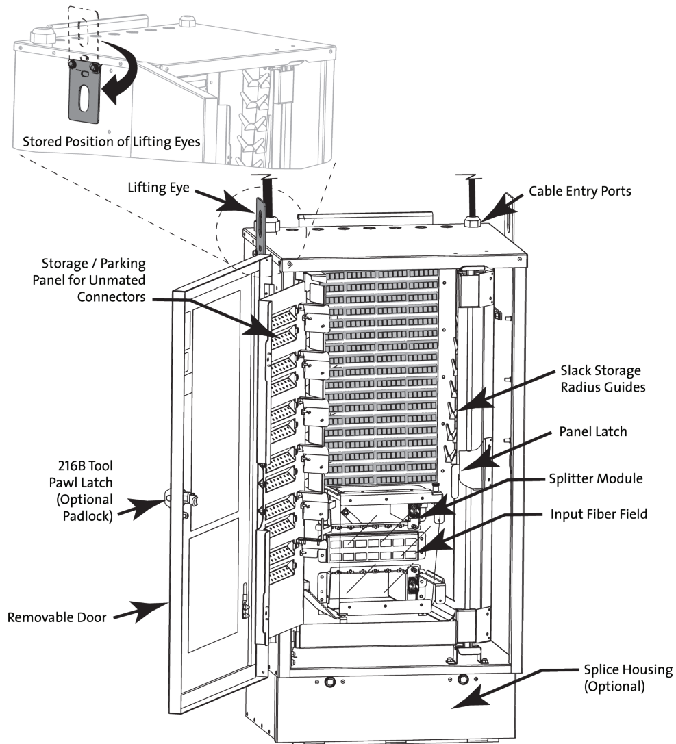
OptiTect Indoor GEN III Cabinet | Drawing ZA-3112
