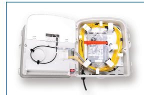
Stubbed MDU Terminal | Photo CRR822
