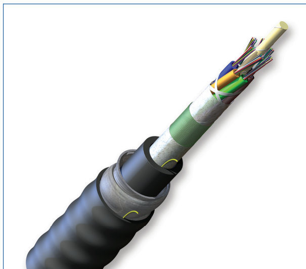
Industrial LSZH Loose Tube, Gel-Free, Interlocking Armored Cables, 72 Fibers | Photo PIM0735
