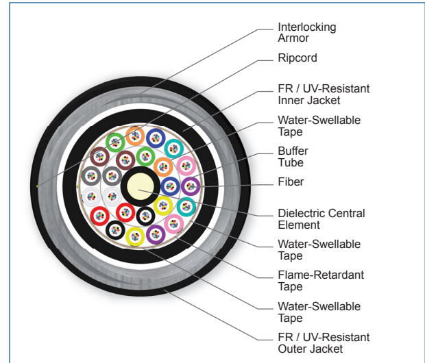
FREEDM Loose Tube Interlocking Armored Cables, 288 Fibers | Photo PIM1717
