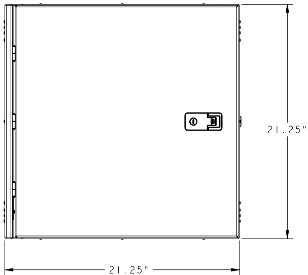
front (closed)
