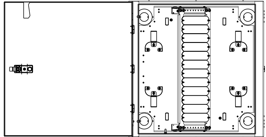
front (open)
