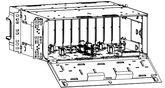
REAR VIEW (WITH DOOR OPEN)
