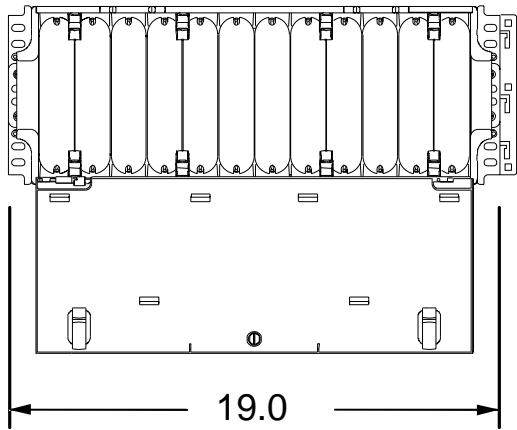
FRONT VIEW (WITH DOOR OPEN)
