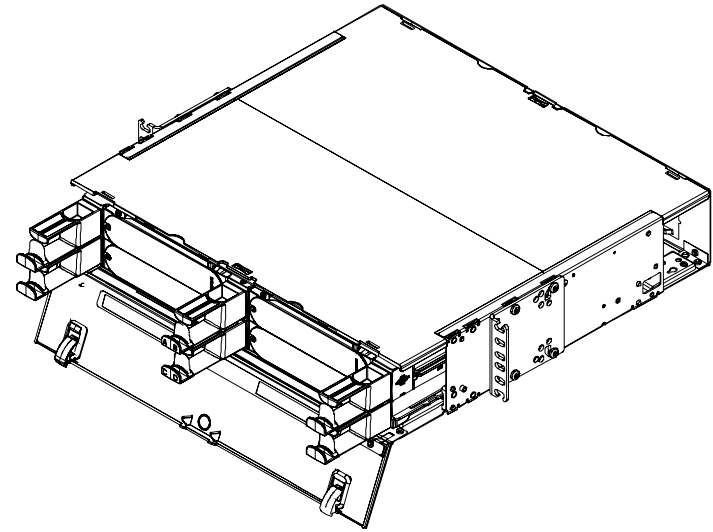
FRONT VIEW (WITH DOOR OPEN)
