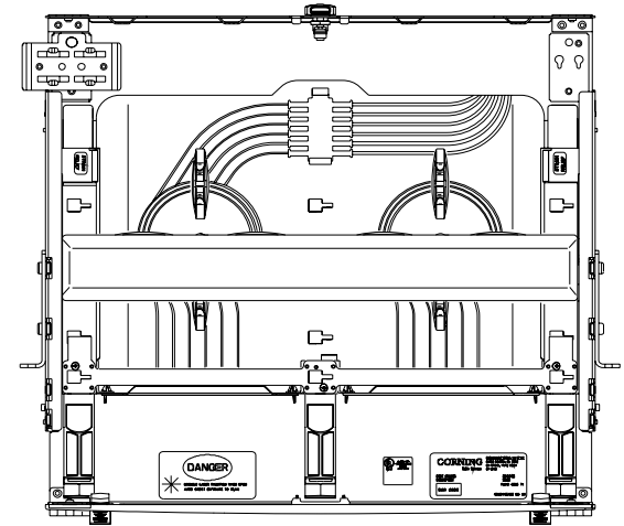
TOP VIEW (WITH COVER REMOVED)
