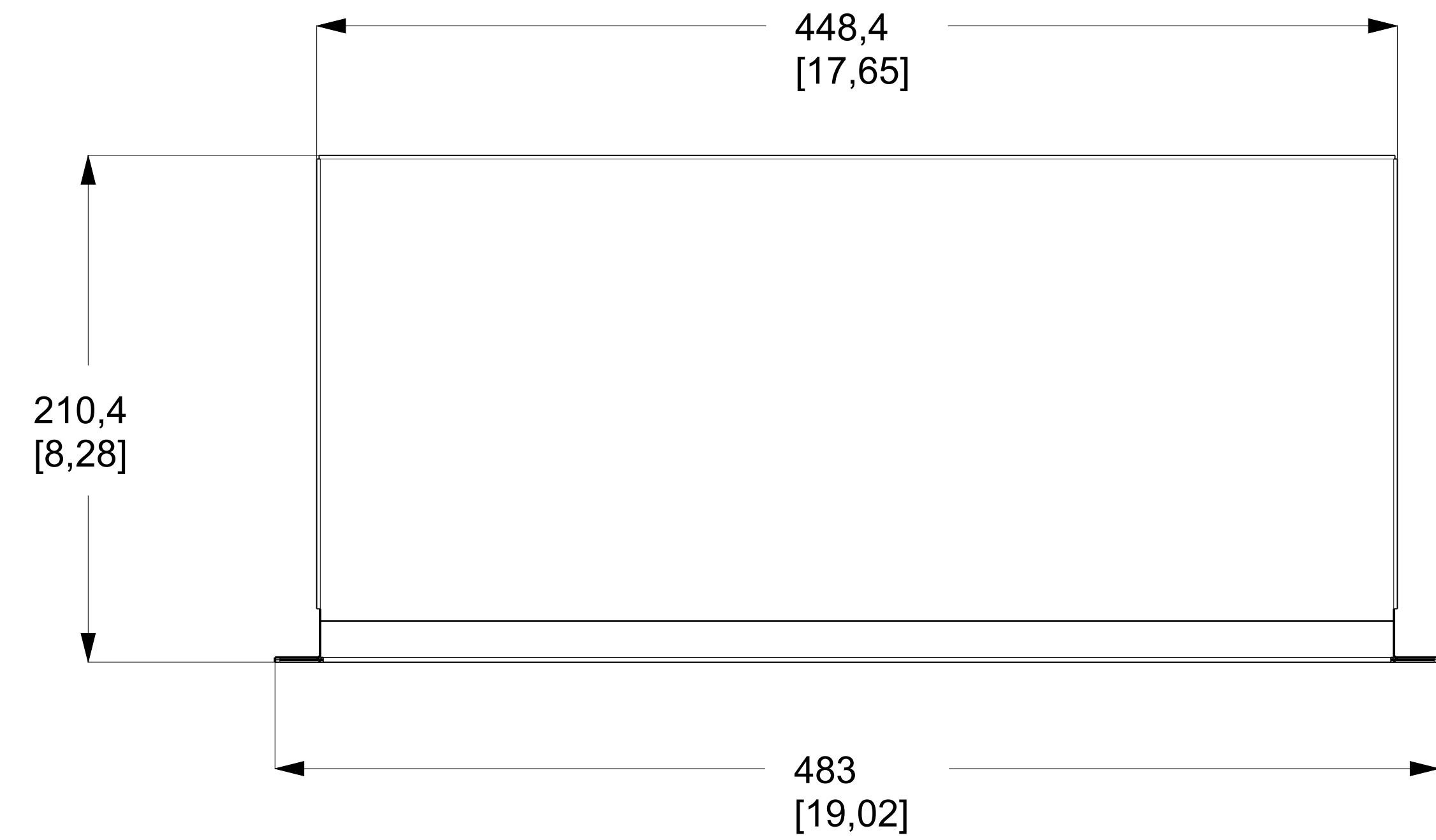
REAR VIEW
