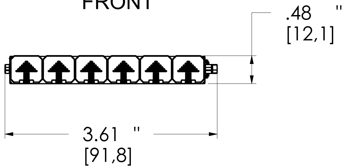
FRONT
