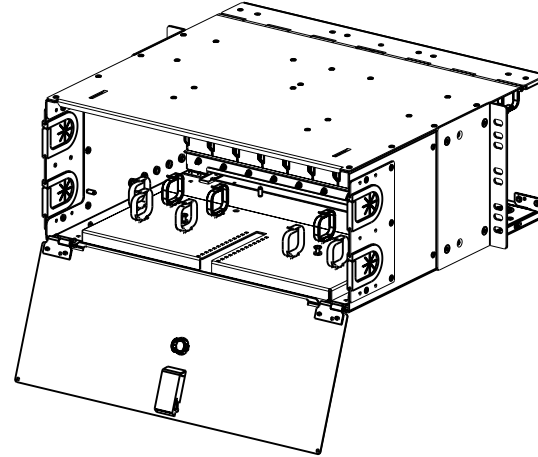
rear (open)
