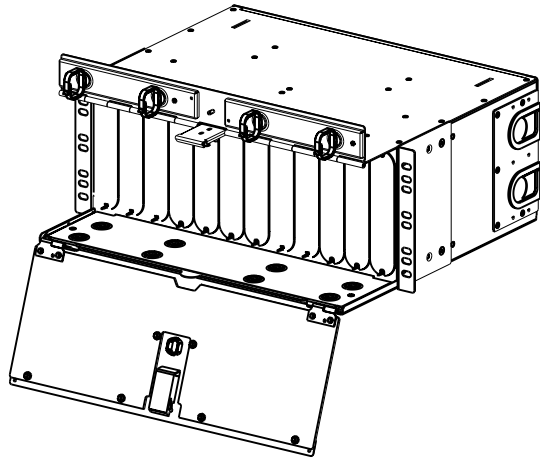
front (open)
