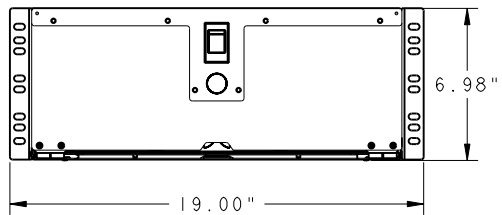
front (closed)
