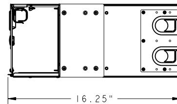
right side
