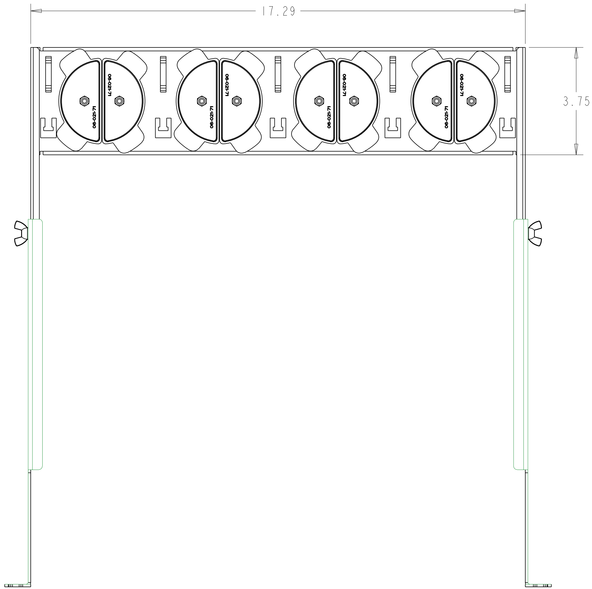
TOP VIEW
