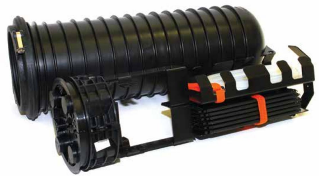
Figure 24. 28-in Splice Canister Closure
