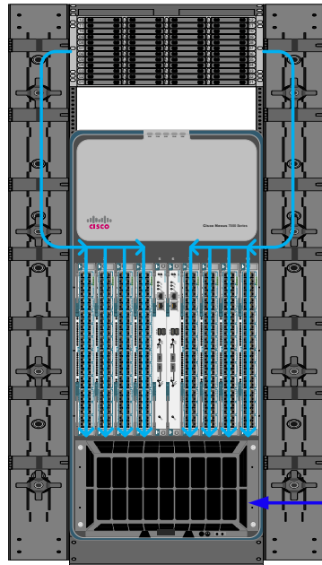
Cabling from the Top
