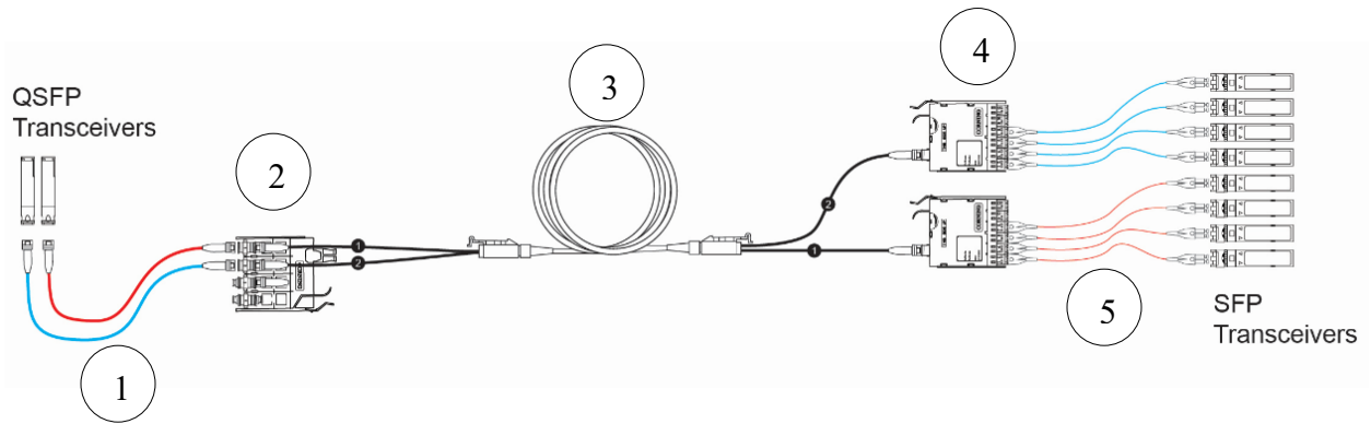
Figure 6: Jumpers, Trunks, Panels, and Modules - Inter-connect Structured Cabling
