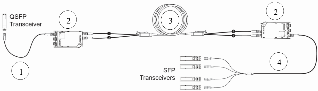
Figure 9: Jumpers, Harnesses, Conversion Modules and Trunks Inter-connect Structured Cabling
