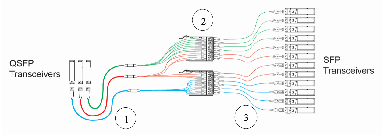
Figure 5: Jumpers, Harnesses and EDGE™ LC/LC Adapter Panel Inter-connect Structured Cabling
