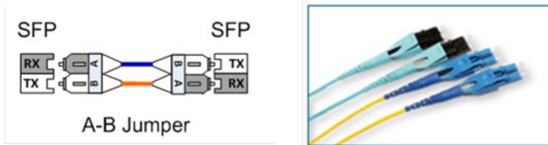
Figure 1: Duplex Fiber Optic Transmission
