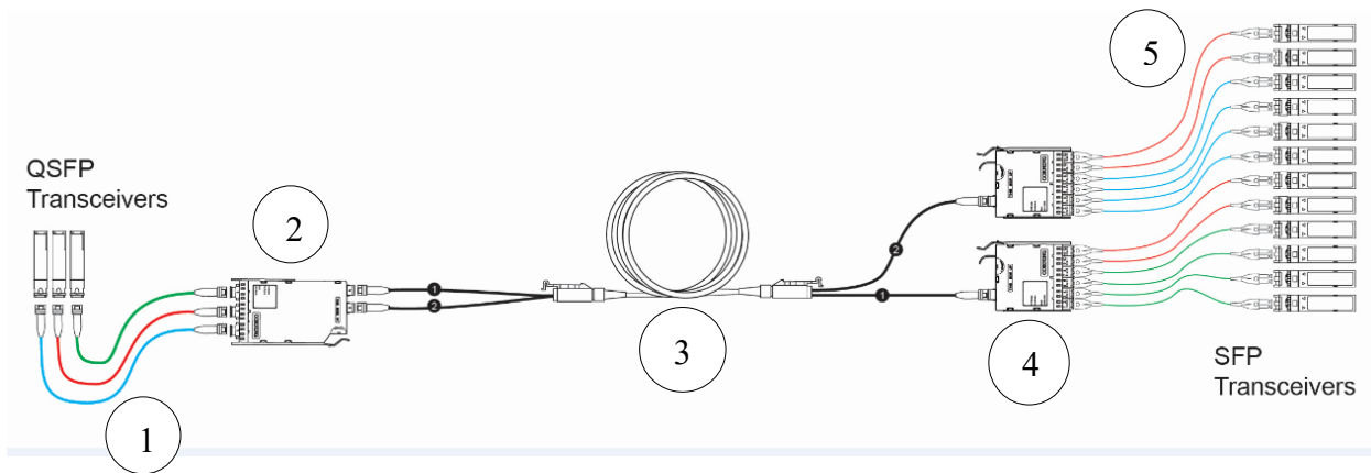
Figure 7: Jumpers, Conversion Modules, Modules, and Trunks Inter-connect Structured Cabling
