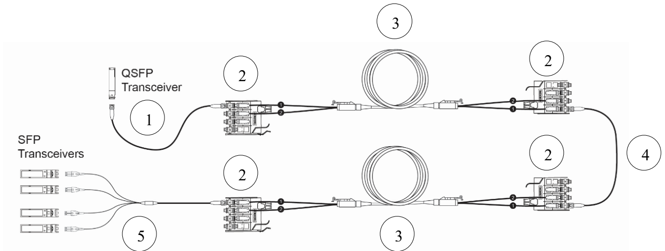
Figure 10: Jumpers, Panels, Trunks, and Harnesses - Cross-connect Structured Cabling
