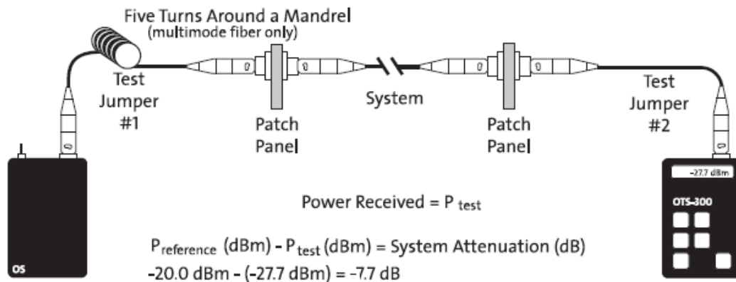
Figure 3: One-jumper End-to-end test
