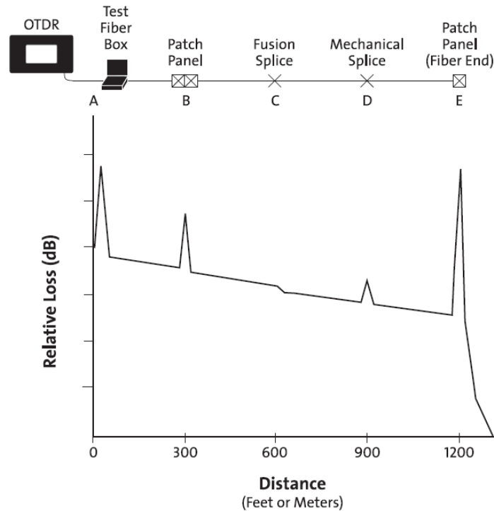
Figure 5: OTDR Test Configuration & Trace
