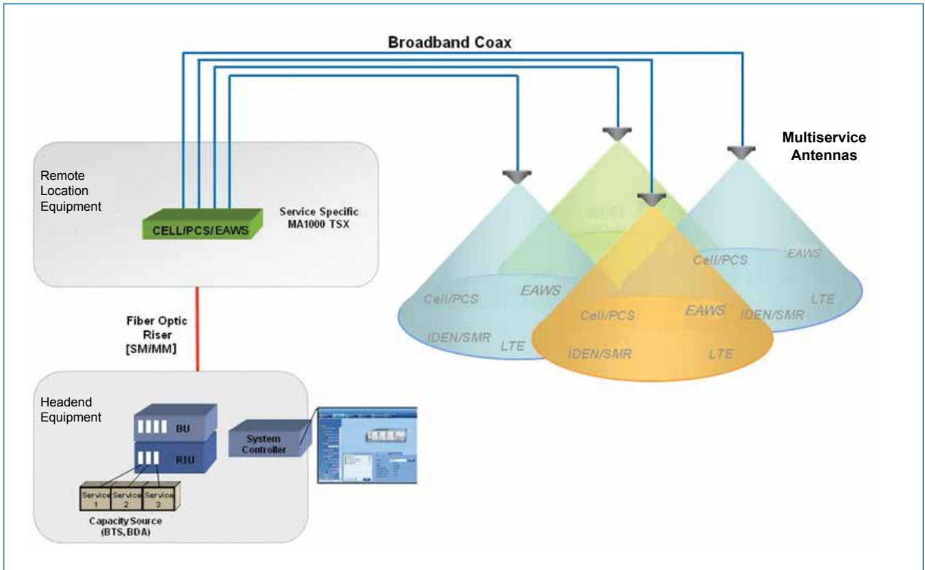
Example of MA1000 System Deployment | Figure 3
