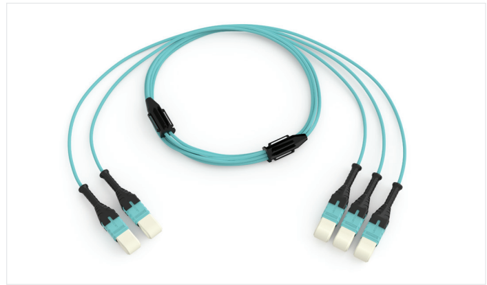
EDGE 2x3 Conversion Harness | Photo REN7929
