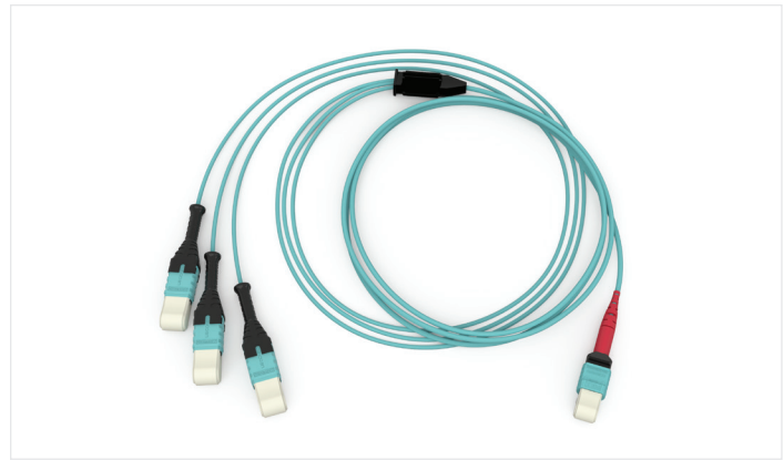
EDGE 24-Fiber MTP Breakout Harness | Photo REN7937
