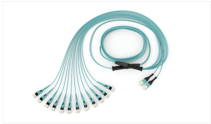
EDGE Hybrid MTP to LC Uniboot Extender Trunk | Photo REN7796
