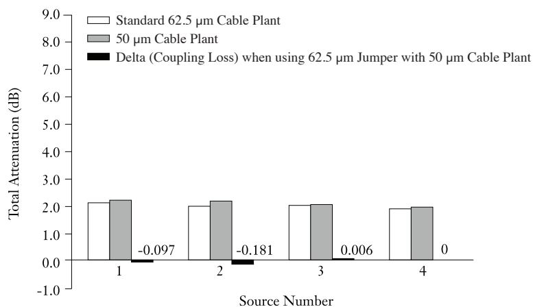
62.5 \mu\text{m} Jumper with 62.5 \mu\text{m} Cable Plant vs 50 \mu\text{m} Cable Plant
